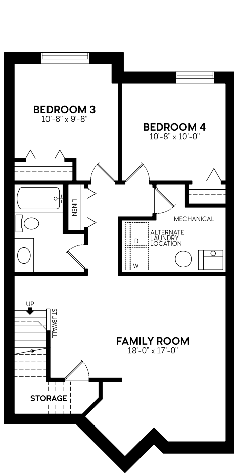
BASEMENT OPTIONAL DEVELOPMENT 720FT 2
